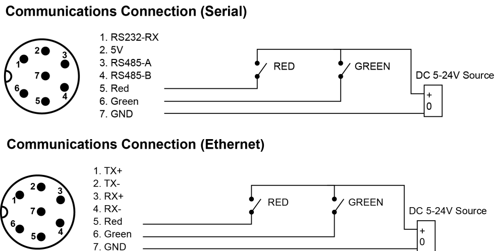
Figure 11: Driving traffic lights from external DC source
