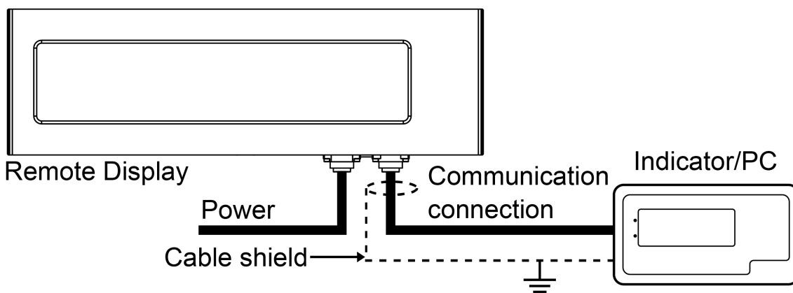
Figure 5: Shield Earthing
