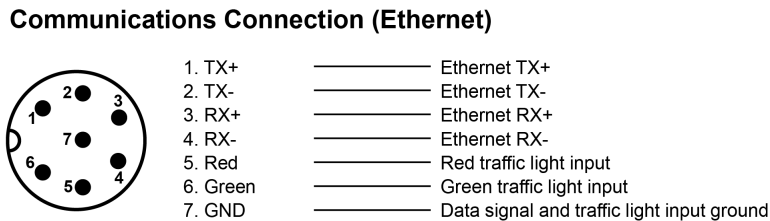
Figure 9: Ethernet socket connections
