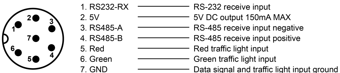
Figure 6: Serial socket connections
