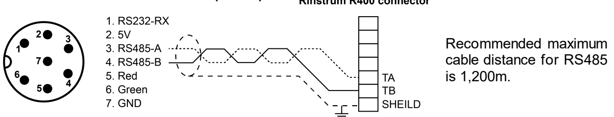
Figure 8: RS485 Socket connection
