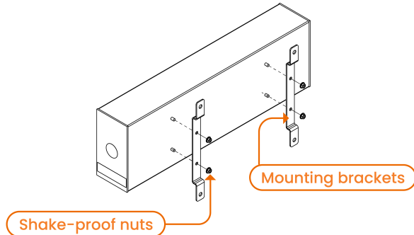
Figure 12: Mounting brackets
