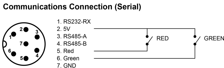
Figure 10: Driving traffic lights from internal 5VDC source
