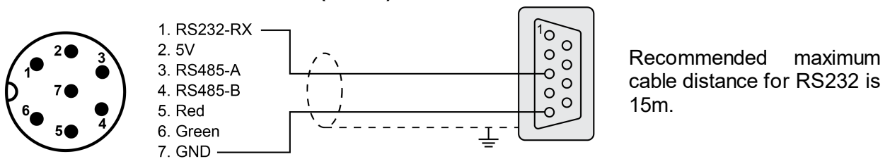
Figure 7: RS232 Socket connection
