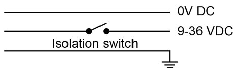
Figure 4: DC power supply socket connection
