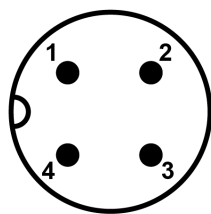
Figure 3: AC power supply socket connection
