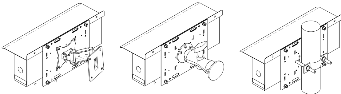
Figure 14: VESA, RAM and Pole mounting examples
